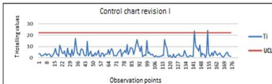
Figure 3. Revision I of control chart T^2 Hotelling
